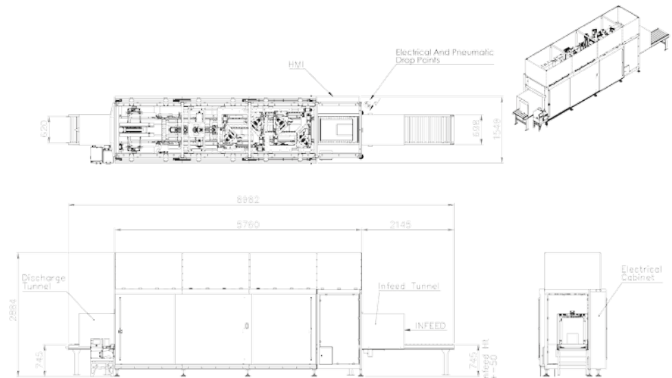
Typical box out cut/ crimp/fold/glue/lid reduced volume 1
